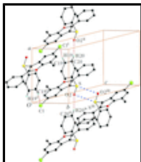
Fig. 2. C–H...O, C–H...Cl, and S...O interactions (dotted lines) in the title compound. [Symmetry code: (i) -x + 1, -y + 1, -z ; (ii) x + 1, y, z ; (iii) -x, -y + 1, -z + 1 ; (iv) -1 + x, y, z .]
